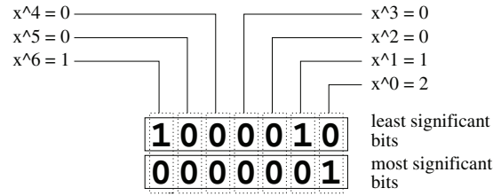
Fig. 1. Bit-sliced Representation
