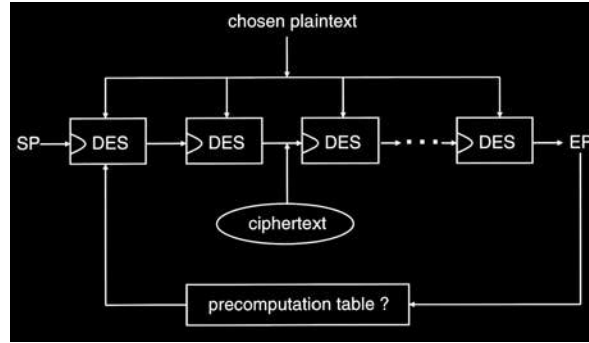
Fig. 2. Online attack
