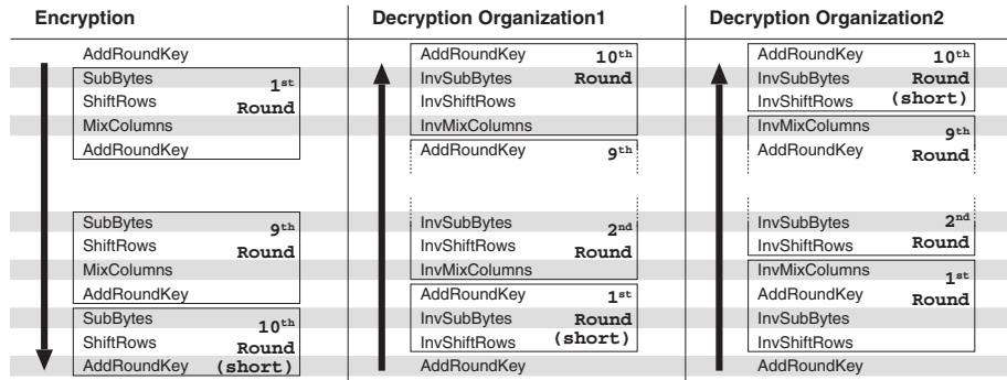
Fig. 5. The two options for delimiting one Rijndael decryption round.
