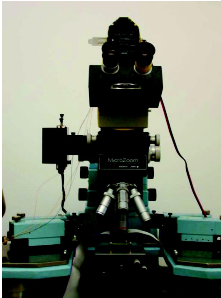
Fig. 3. Wentworth Labs MP-901 manual probe with Vivitar 550FD photoflash lamp mounted on top
