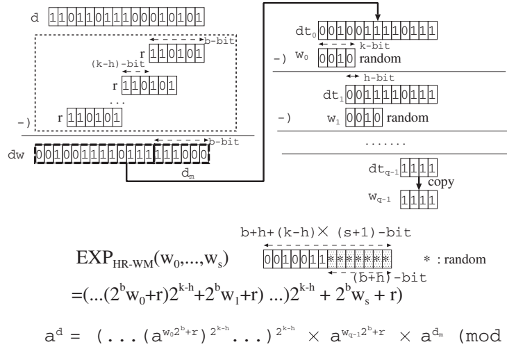
Fig. 3. Overview of HR-WM and EXP_{HR-WM}(w_0, \dots, w_s)
