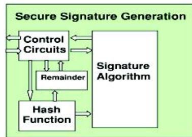
Fig. 1. Top Level Architecture.
