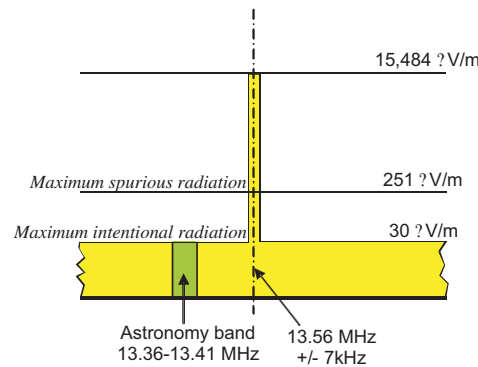
Fig. 2. The 13.56 MHz ISM band US power regulations.
