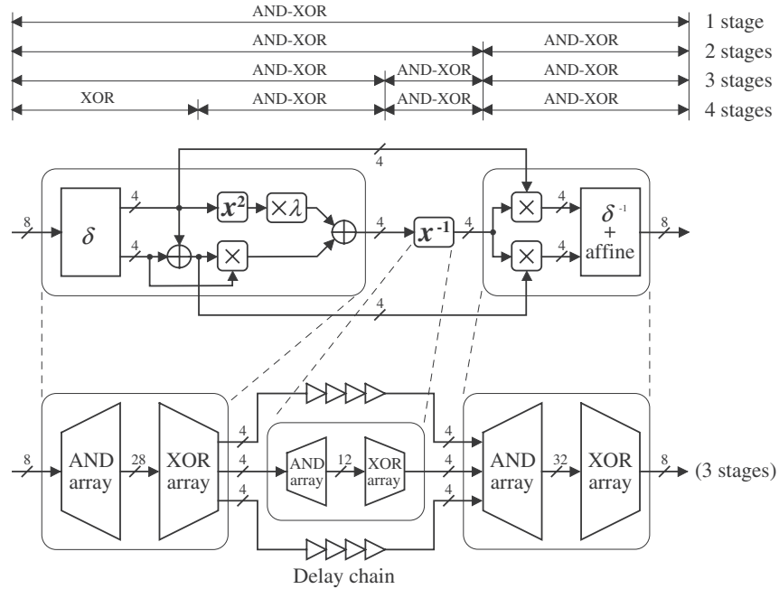
Fig. 5. A conventional composite field S-Box (top) and the proposed method called multi-stage PPRM (bottom)
