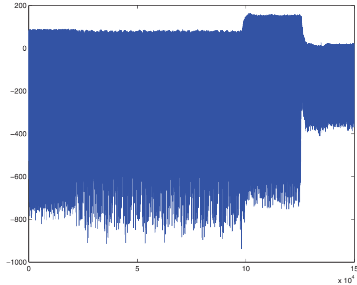
Fig. 11. Average signal showing details of checksum calculation for 8 key bytes.
