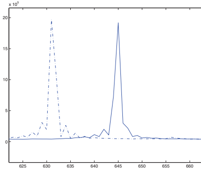
Fig. 4. Two FFTs showing loop frequency differences (LSB 0 and 1) for smartcard A
