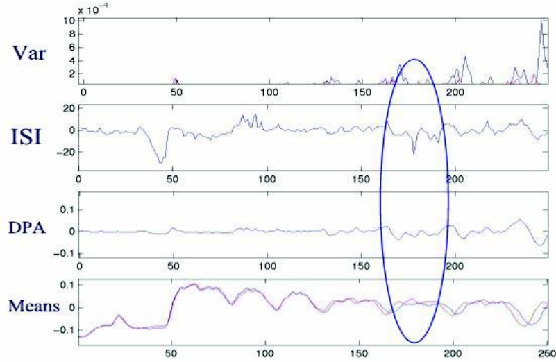
Fig. 5. Variances, ISI_{sn}(t)^{-1} , DPA, and means of WRI
