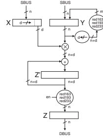
Fig. 7. Least-Significant-Digit-First Multiplier.
