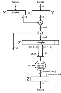
Fig. 6. Shift-and-Add Multiplier.
