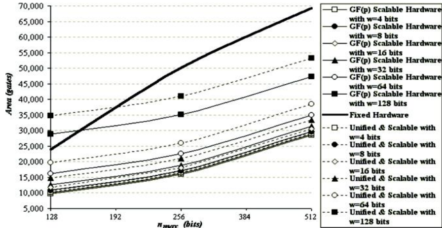
Fig. 9. Area comparison
