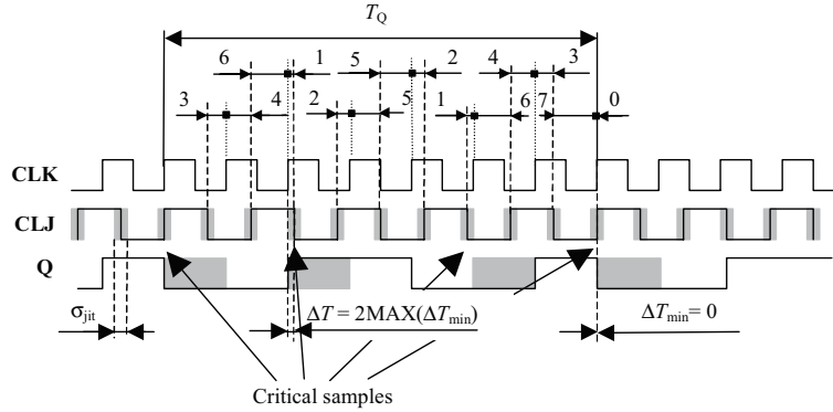
Fig. 5. Clock relation for K_M = 5 , K_D = 7 ( F_{\text{CLJ}} < F_{\text{CLK}} )
