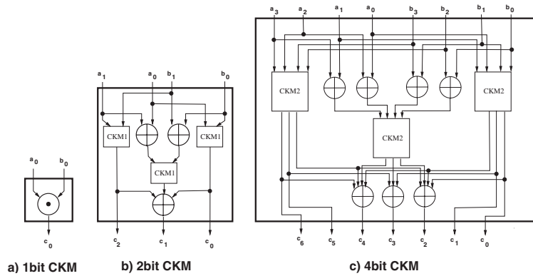
Fig. 3. Recursive construction process for CKM
