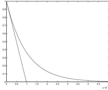
Fig. 4. Linear approximation of (1-x)^k with k = 2^{10}
